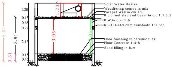
SECTION - "AB "
