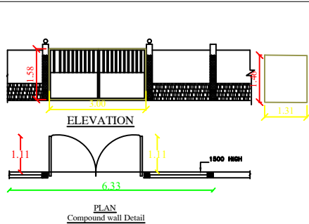
Compound wall Detail
