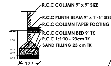
SECTION COLUMN DETAILS PLAN
