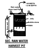
SEC. RAIN WATER HARVEST PIT
