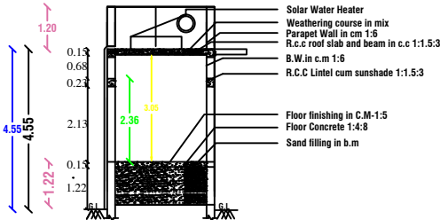
SECTION - "AB "
