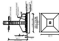
FOUNDATION DETAILS
