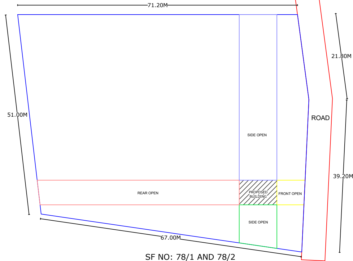
SITE PLAN: NOT TO SCALE
