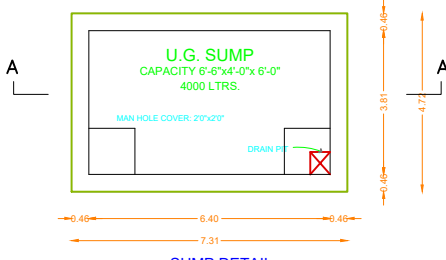
SUMP DETAIL
