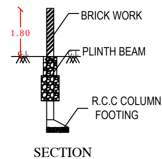
SECTION
