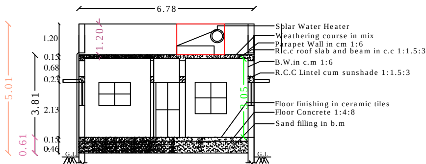
SECTION - "AB "
