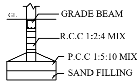
COLUMN DETAILS
