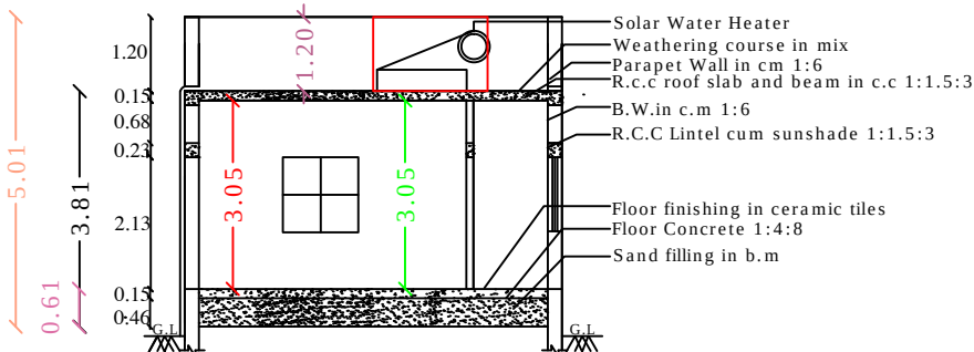
SECTION - "AB "
