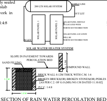
SECTION OF RAIN WATER PERCOLATION BED
