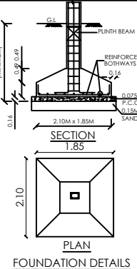
FOUNDATION DETAILS
