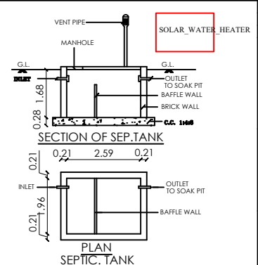
PLAN SEPTIC TANK
