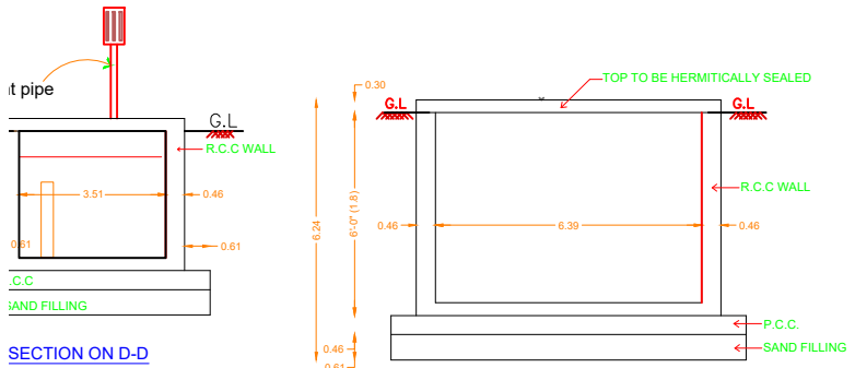
SECTION ON D-D
