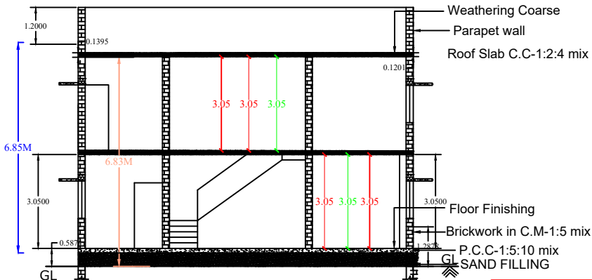
CROSS SECTION ON AB
