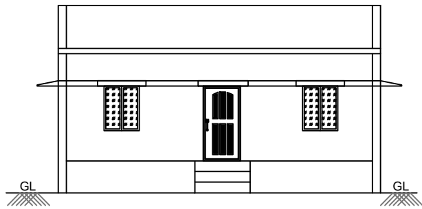
FRONT ELEVATION (SCALE 1:150)
