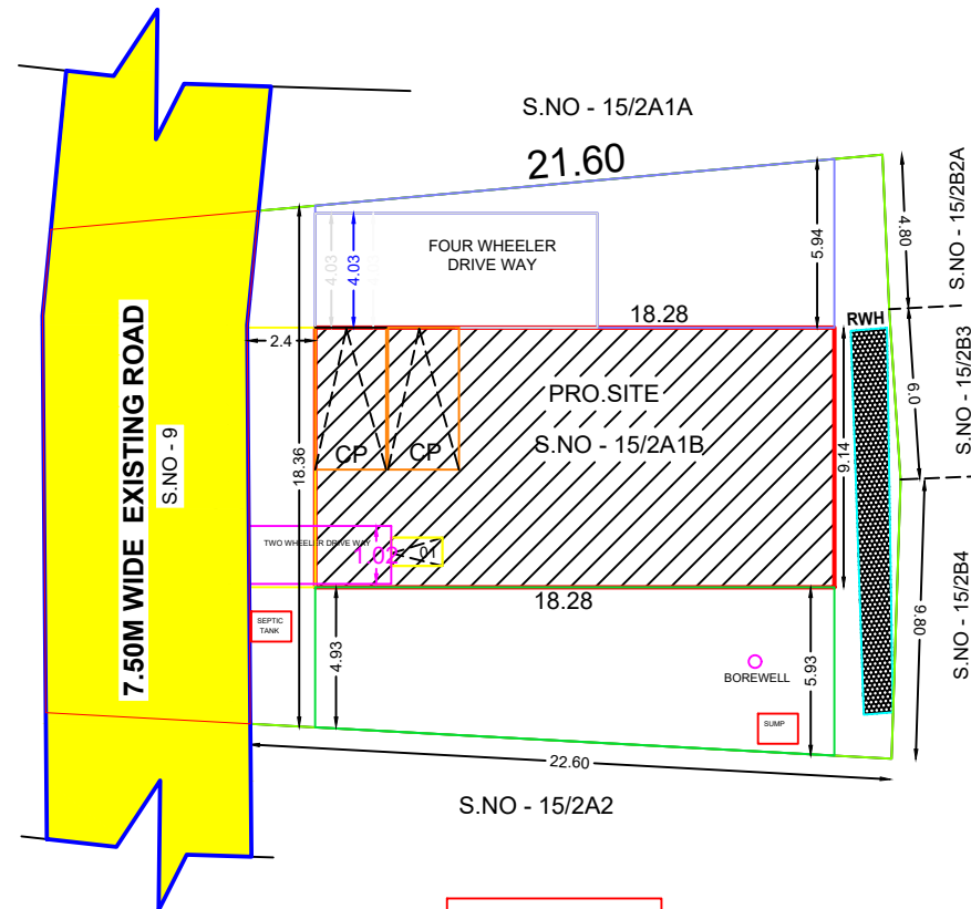
SITE PLAN
