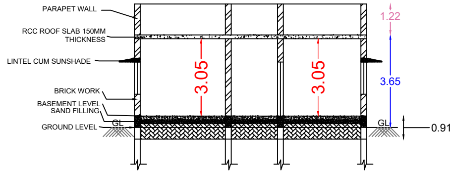
SECTION ON XX (SCALE 1:150)
