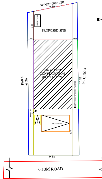
SITE PLAN
