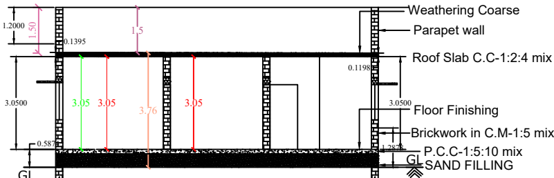
CROSS SECTION ON AB
