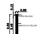
DETAILS OF PERCULATION PIT
