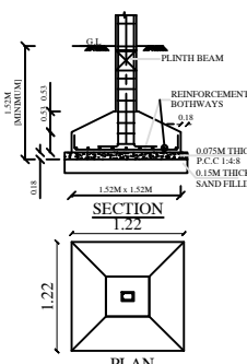
FOUNDATION DETAILS
