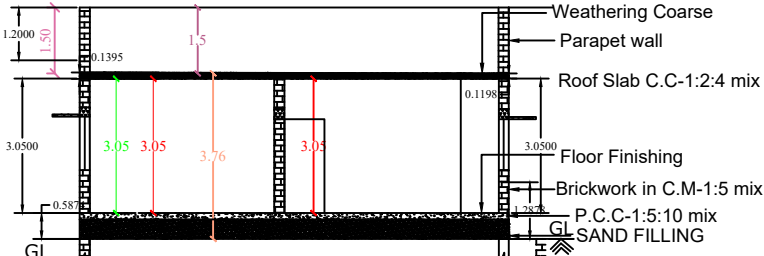
CROSS SECTION ON XX
