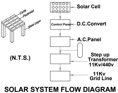
SOLAR SYSTEM FLOW DIAGRAM
