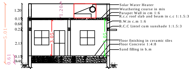
SECTION - "AB "
