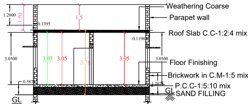
CROSS SECTION ON XX
