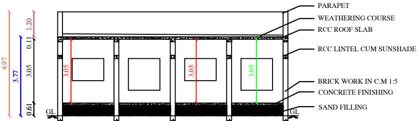
SECTION ON AB
