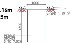
SECTION OF PEBBLE TRENCH
