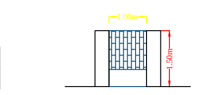
WICKET GATE
