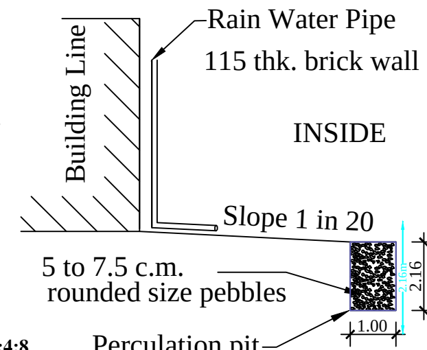
RAIN WATER HARVESTING PERCOLATION PIT RWH_CAPACITY_L=2000LTRS
