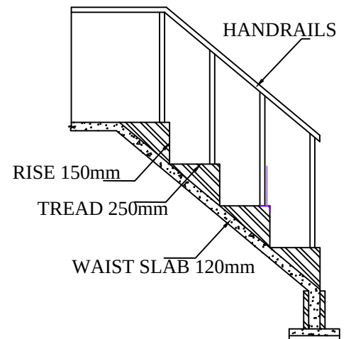
STAIRCASE DETAILS
