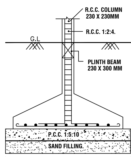
FOUNDATION DETAIL
