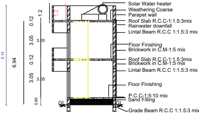
SECTION ON A,B & C,D
