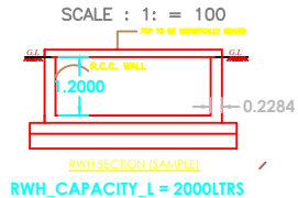
RW SECTION SAMPLE
