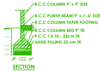
SECTION
