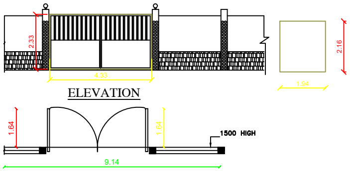
PLAN Compound wall Detail
