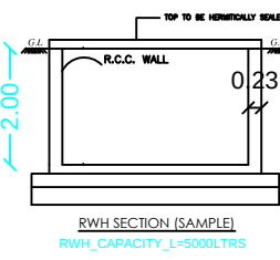
RWH SECTION (SAMPLE) RWH_CAPACITY_1=5000LTS
