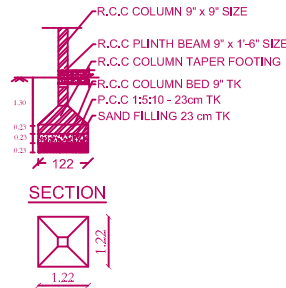
COLUMN DETAILS PLAN
