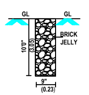
PERCULATION PIT
