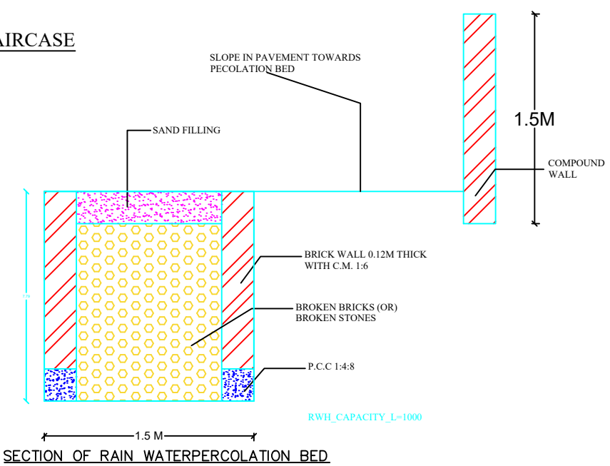
SECTION OF RAIN WATERPERCULATION BED
