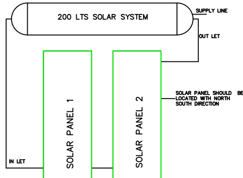
SOLAR WATER HEATER SYSTEM
