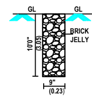
PERCOLATION PIT
