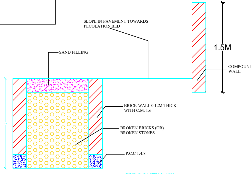
SECTION OF RAIN WATER PERCOLATION BED
