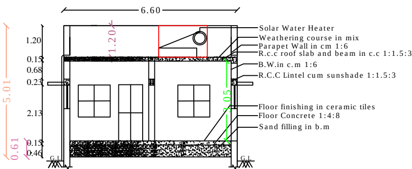
SECTION - "AB "
