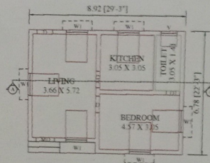
PROPOSED GROUND FLOOR PLAN
