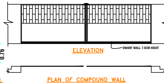
PLAN OF COMPOUND WALL
