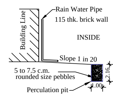
RAIN WATER HARVESTING PERCOLATION PIT RWH_CAPACITY_L=2000LTRS
