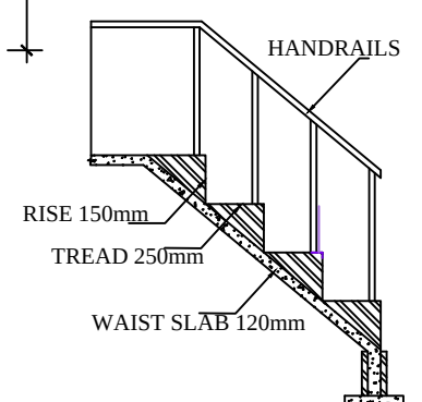
STAIRCASE DETAILS
