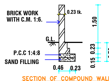
SECTION OF COMPOUND WALL
