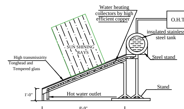
SECTION SOLAR WATER HEATER
