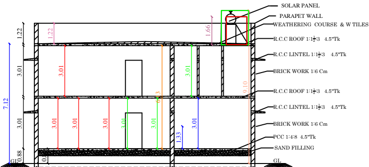
CUT SECTION ON AA
