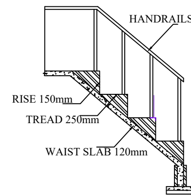
STAIRCASE DETAILS
