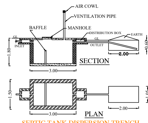
SEPTIC TANK DISPERSION TRENCH
