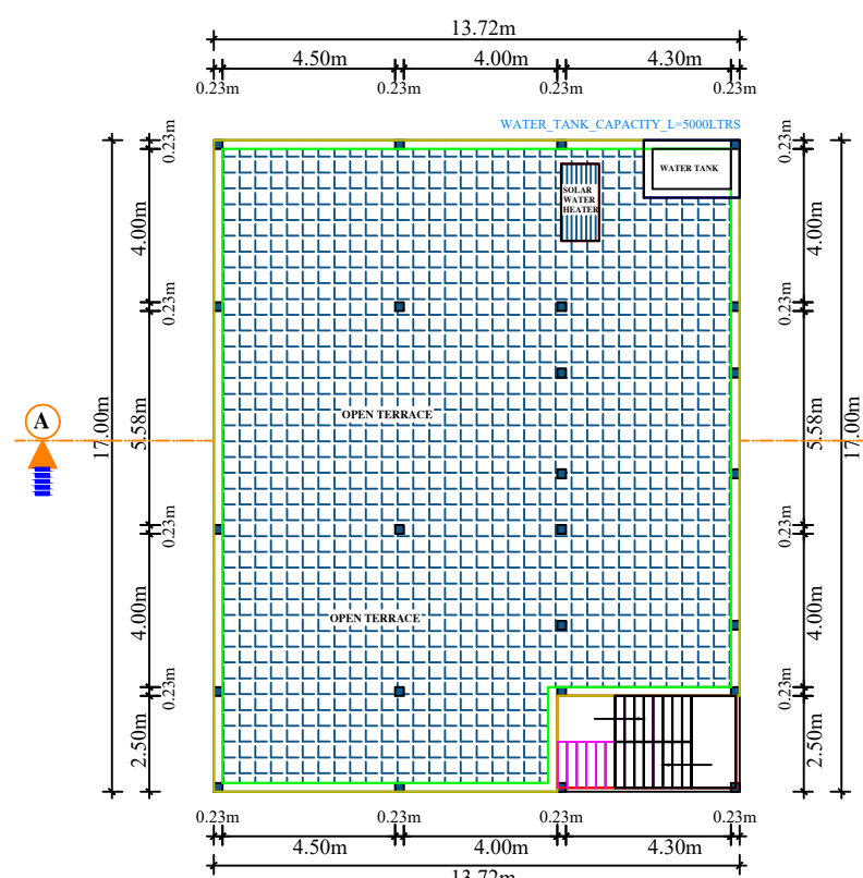
TERRACE PLAN
