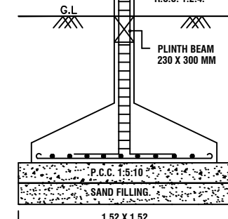
FOUNDATION DETAIL
