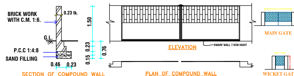
PLAN OF COMPOUND WALL
