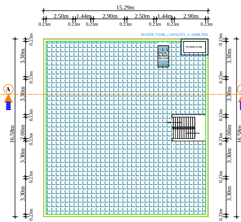
TERRACE PLAN
