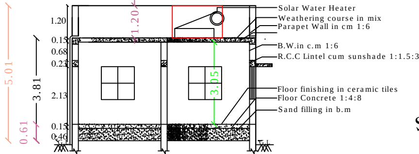
SECTION - "AB "
