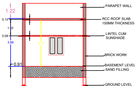
SECTION (AB)
