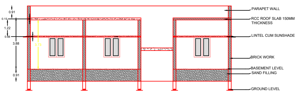
SECTION (A1B1)
