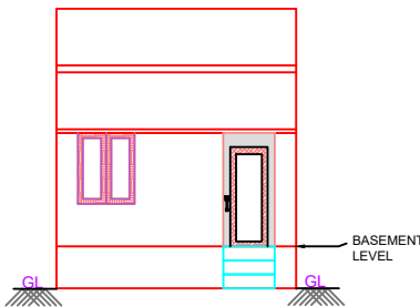
ELEVATION BLOCK-B
