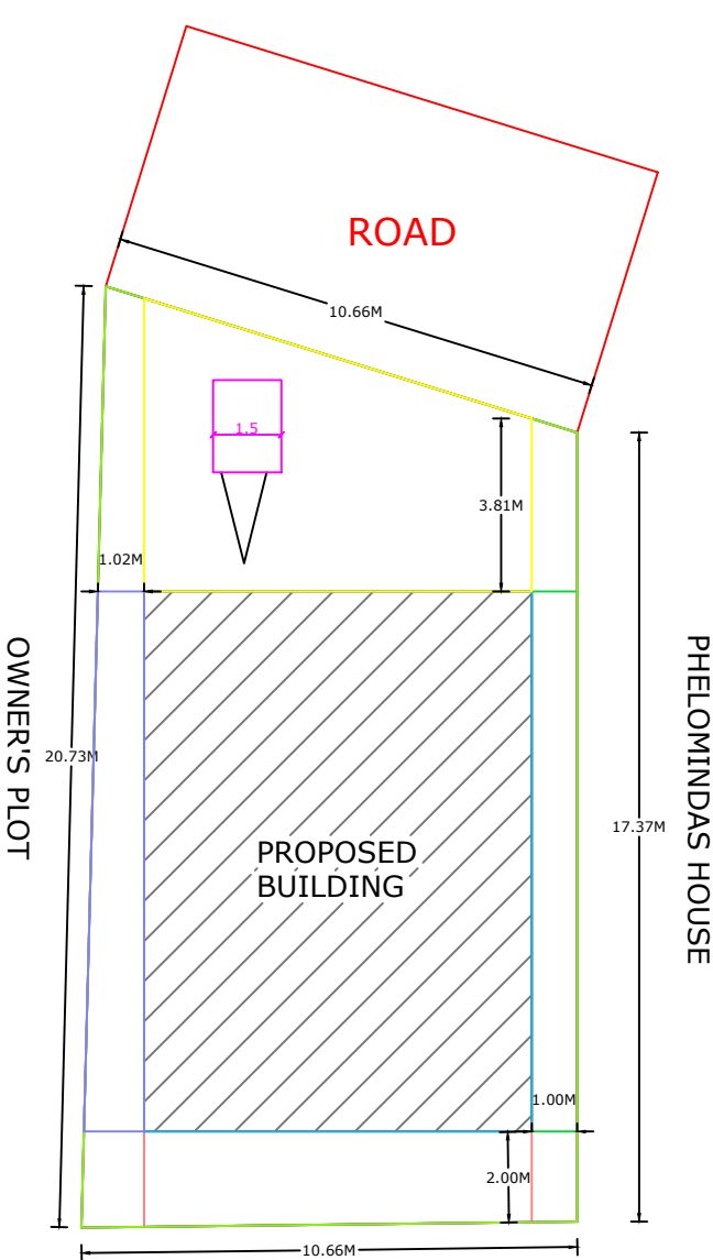
OWNER'S HOUSE SITE PLAN: 1:100
