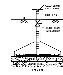
FOUNDATION DETAIL
