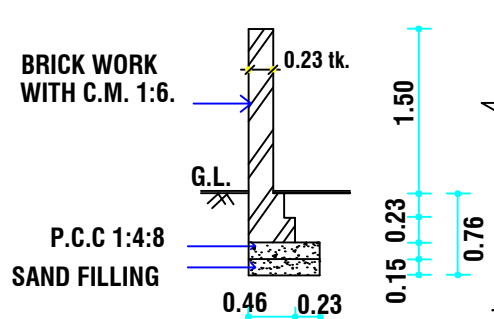
SECTION OF COMPOUND WALL
