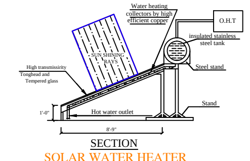
SECTION SOLAR WATER HEATER
