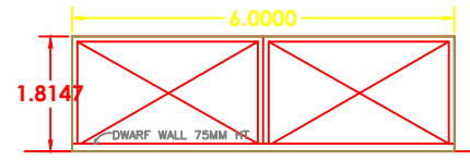
MAIN GATE
