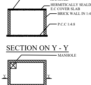
UG - SUMP DETAIL PLAN
