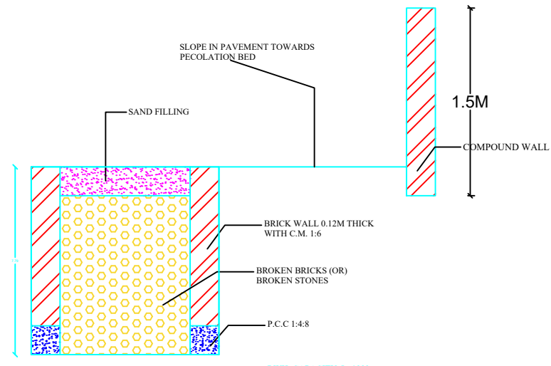
SECTION OF RAIN WATERPERCOLATION BED
