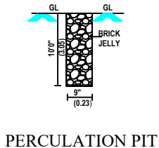
PERCOLATION PIT
