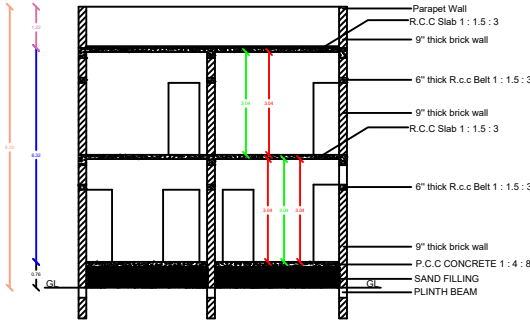
SECTION A - B
