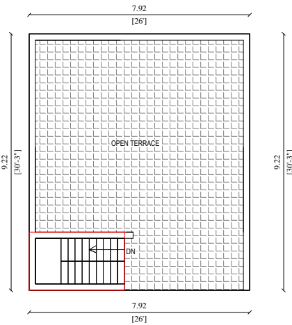
PRO.TERRACE FLOOR
