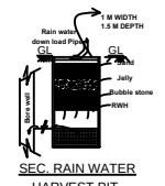
SEC. RAIN WATER HARVEST PIT
