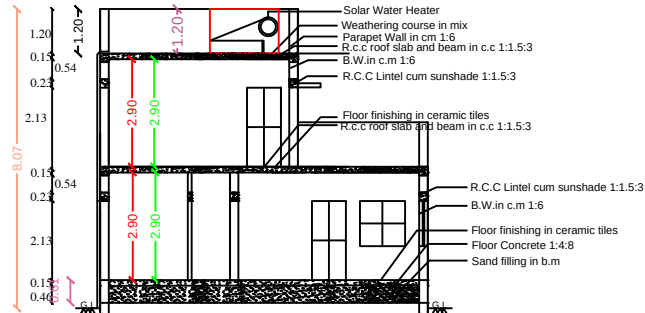
SECTION - "AB - CD "
