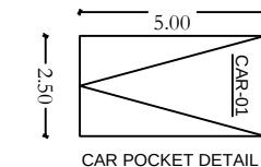
CAR POCKET DETAIL
