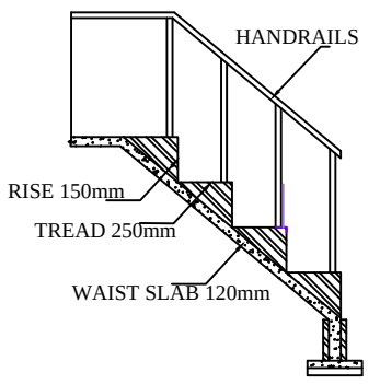
STAIRCASE DETAILS
