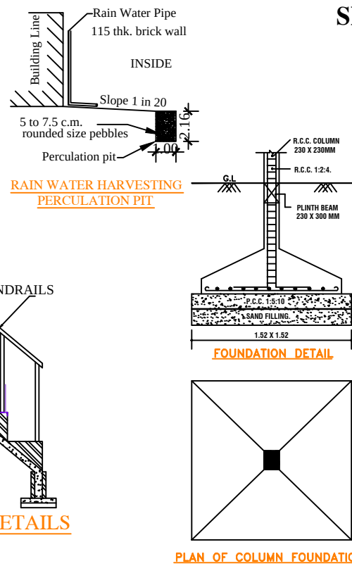
PLAN OF COLUMN FOUNDATION
