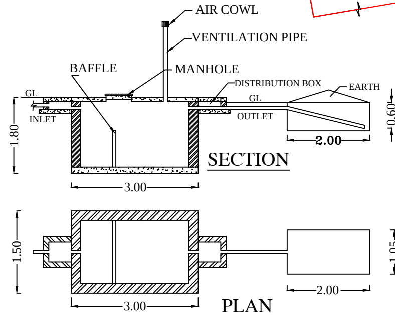
SEPTIC TANK DISPERSION TRENCH
