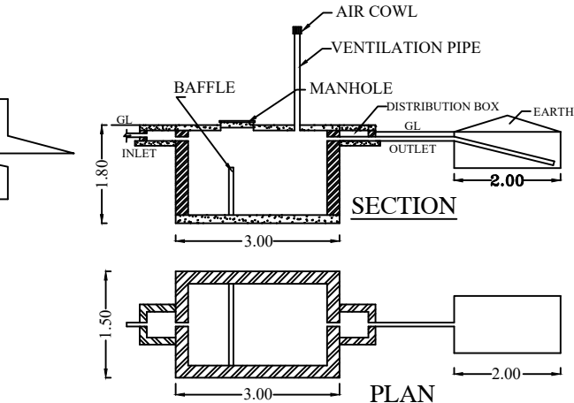
SEPTIC TANK DISPERSION TRENCH
