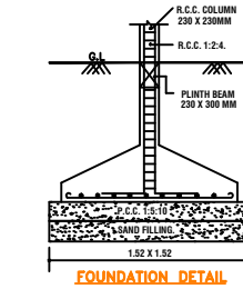
FOUNDATION DETAIL
