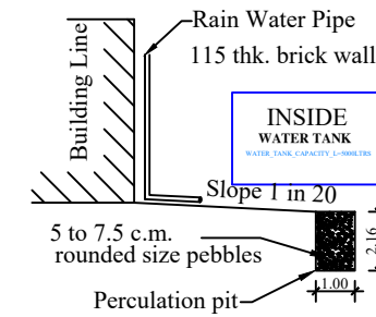
RAIN WATER HARVESTING PERCOLATION PIT
