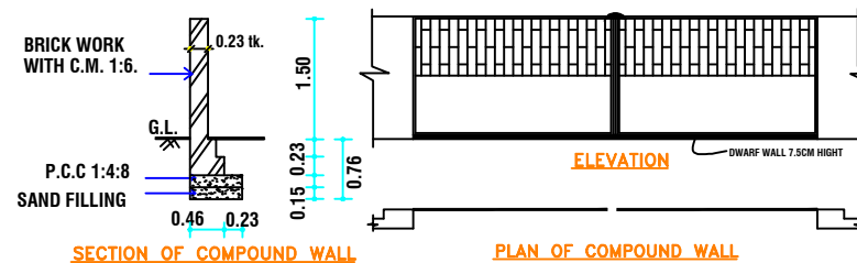
SECTION OF COMPOUND WALL
