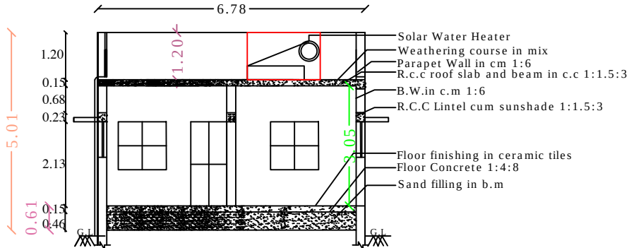
SECTION - "AB "
