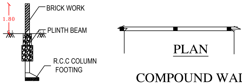
COMPOUND WALL
