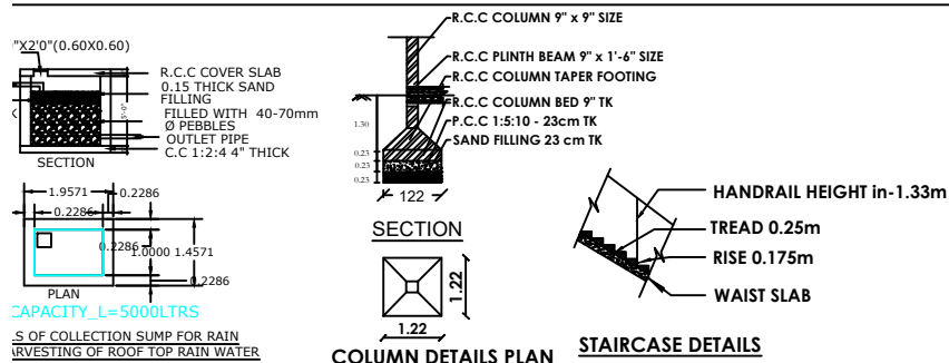
COLUMN DETAILS PLAN
