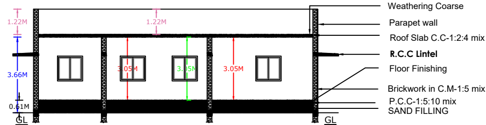
SECTION ON XX
