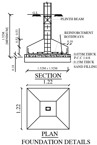
FOUNDATION DETAILS
